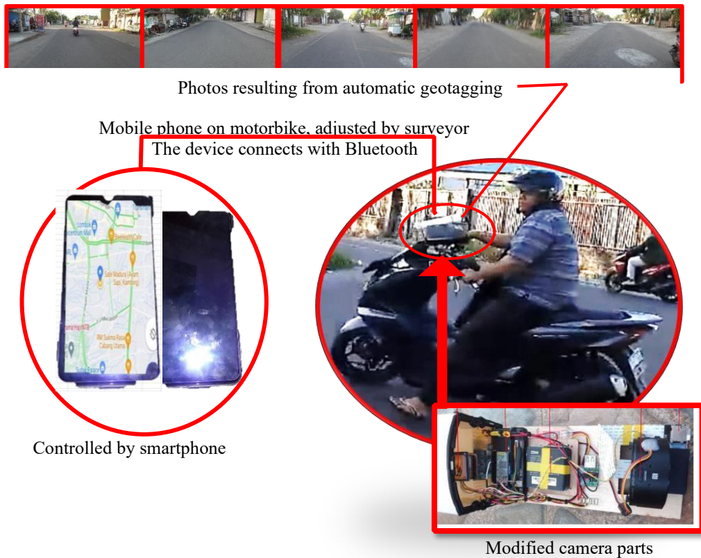
Fig. 2. A set of road condition survey equipment.
