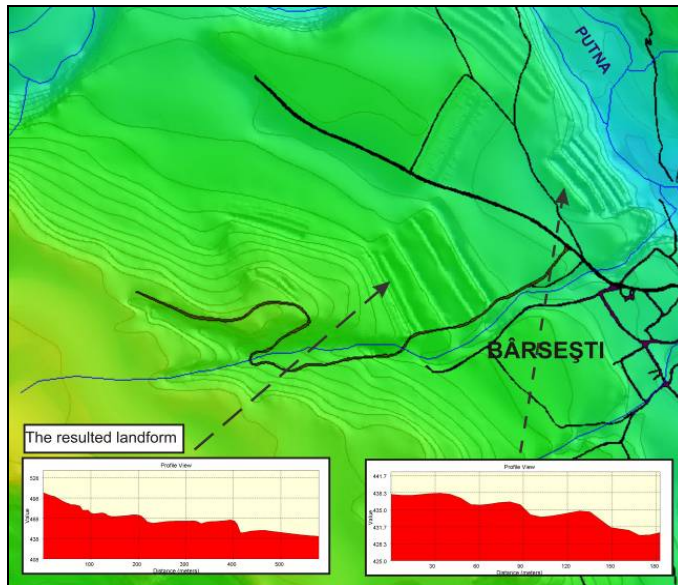
Fig. 4 Agricultural terraces system - Bârsești area; Anthropogenic landforms most easily to represented are agricultural terraces. We choose a representative sample in Bârsești village, where agroterraces were a way to exploit the full potential of the land. Methodology used to achieve these anthropogenic landforms is relatively simple consisting of adding altitude contour lines with values equal to the contour to create forms typical terrace. To highlight the results we have added two longitudinal profiles.
